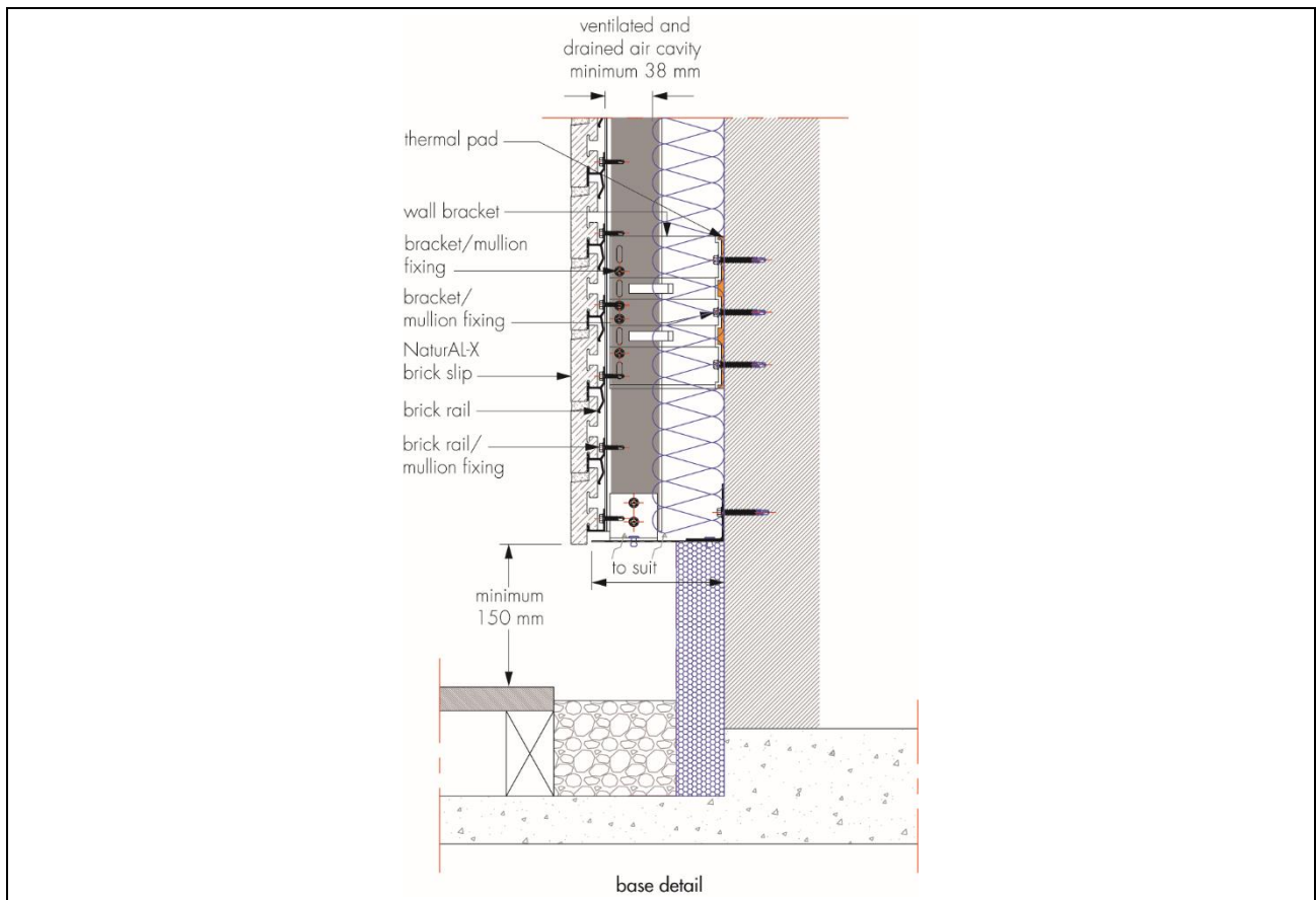
Figure 10 Typical installation base detail
