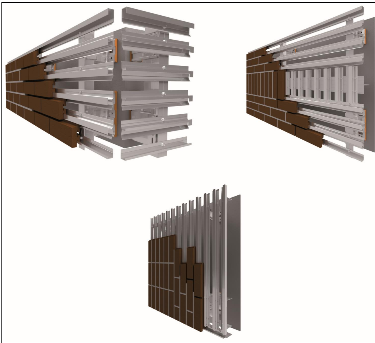
Figure 1 NaturAL-X System and AxiAL Supporting System
