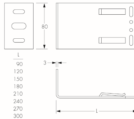
Single Stainless Steel HBS Bracket
