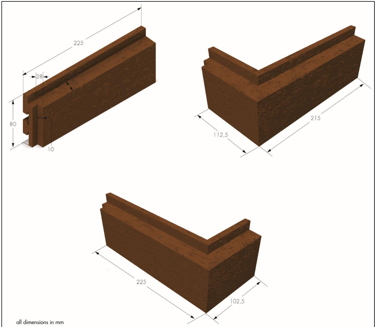
Figure 2 Profiled brick slips
