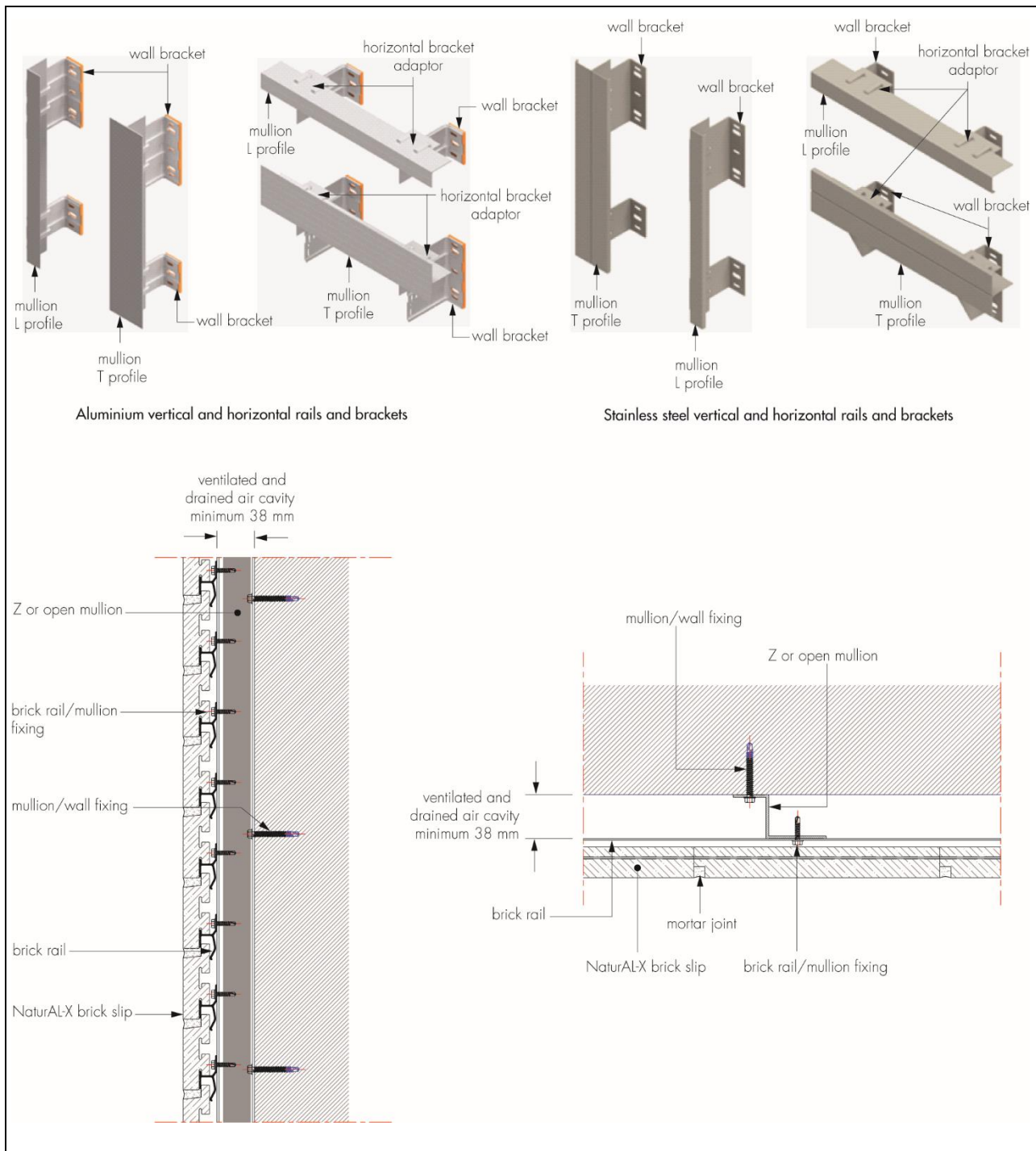
Figure 4 AxiAL Supporting System
