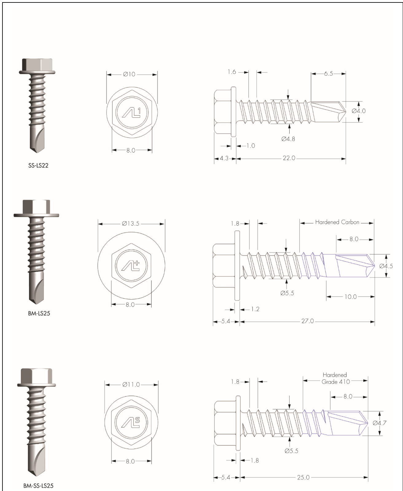
Figure 7 Self-drilling screws
