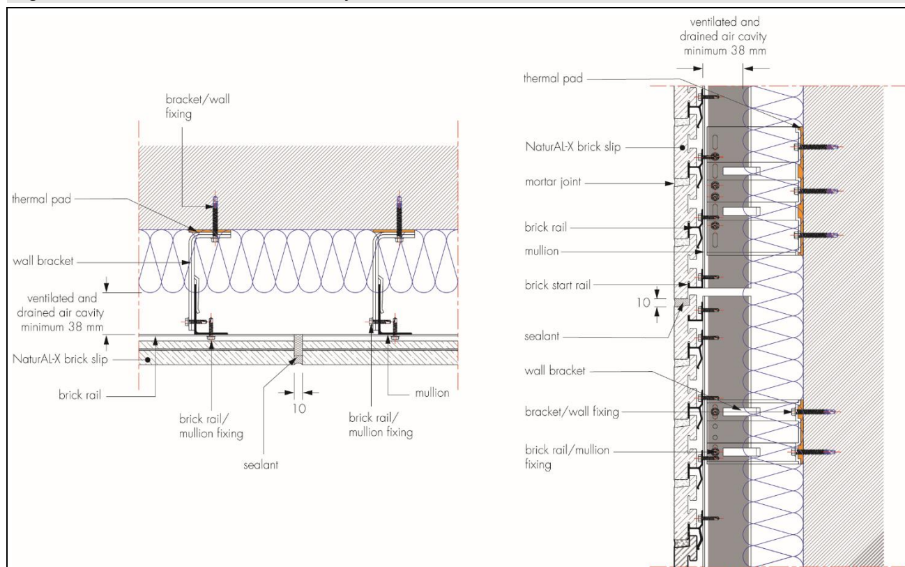
Figure 8 Vertical and horizontal movement joint
