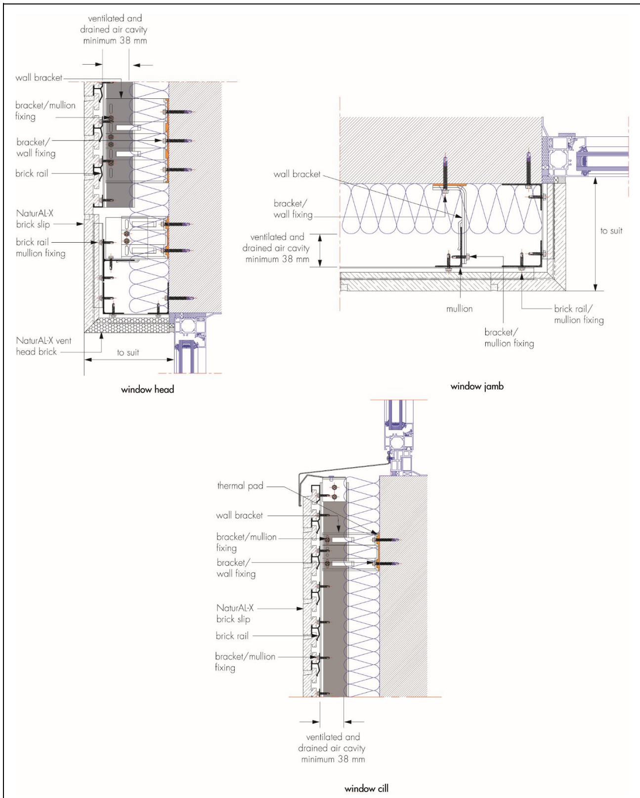
Figure 9 Typical installation detail of the window
