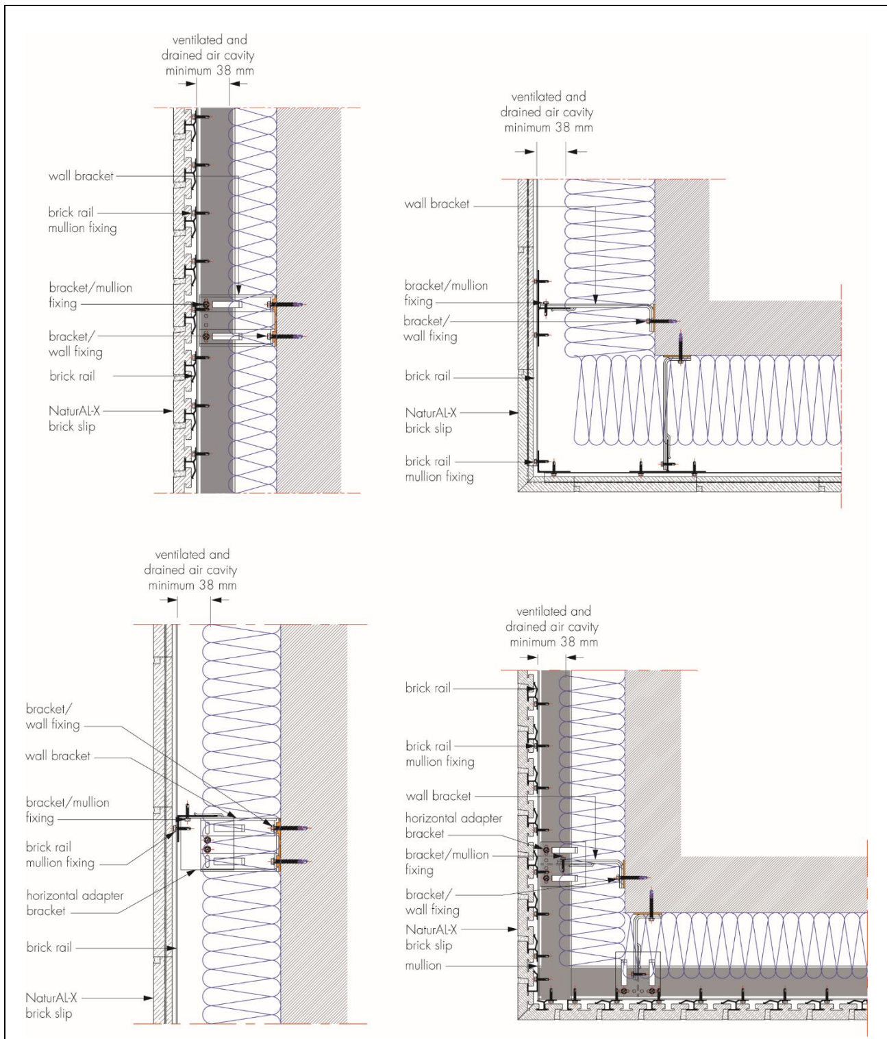
Figure 12 Installation detail of the NaturAL-X Cladding System
