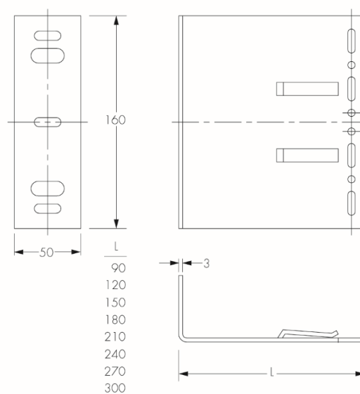
Double Stainless Steel HBS Bracket
