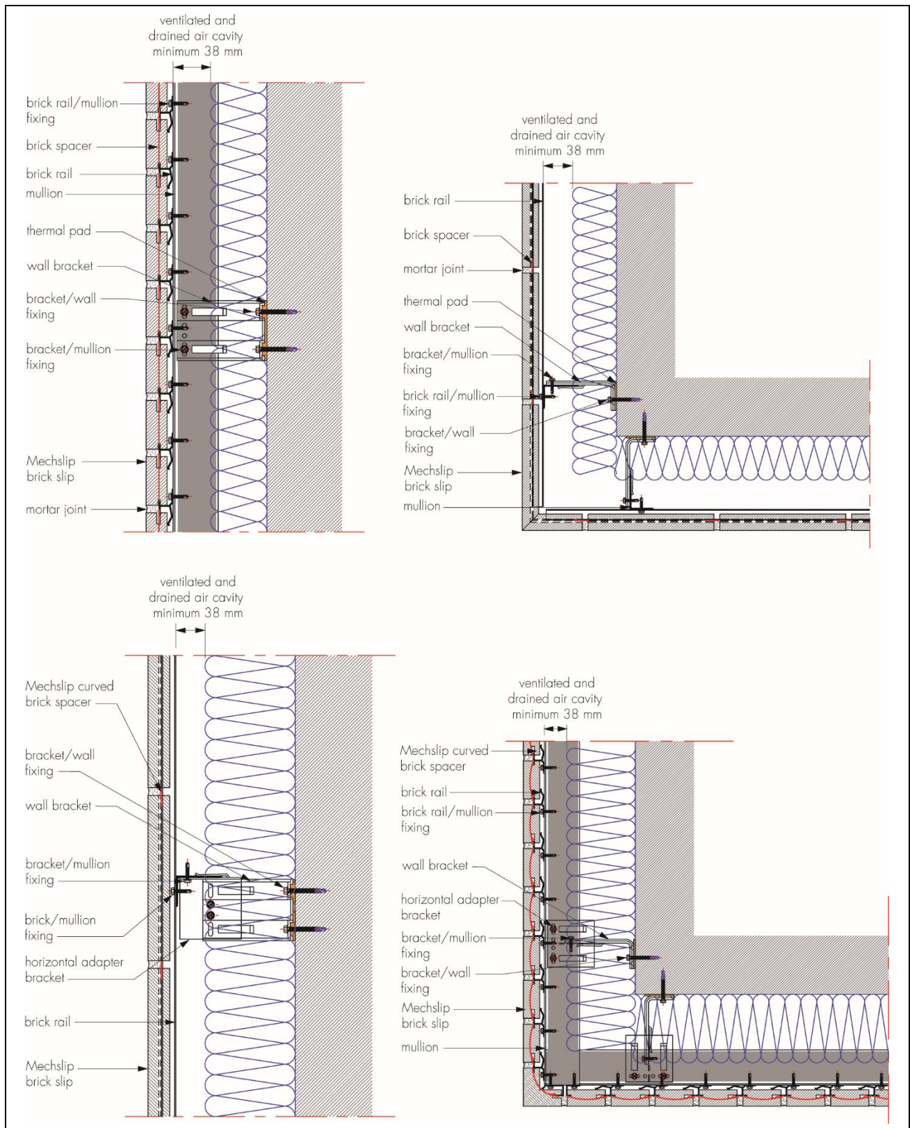
Figure 12 Installation detail of the Mechslip Cladding System
