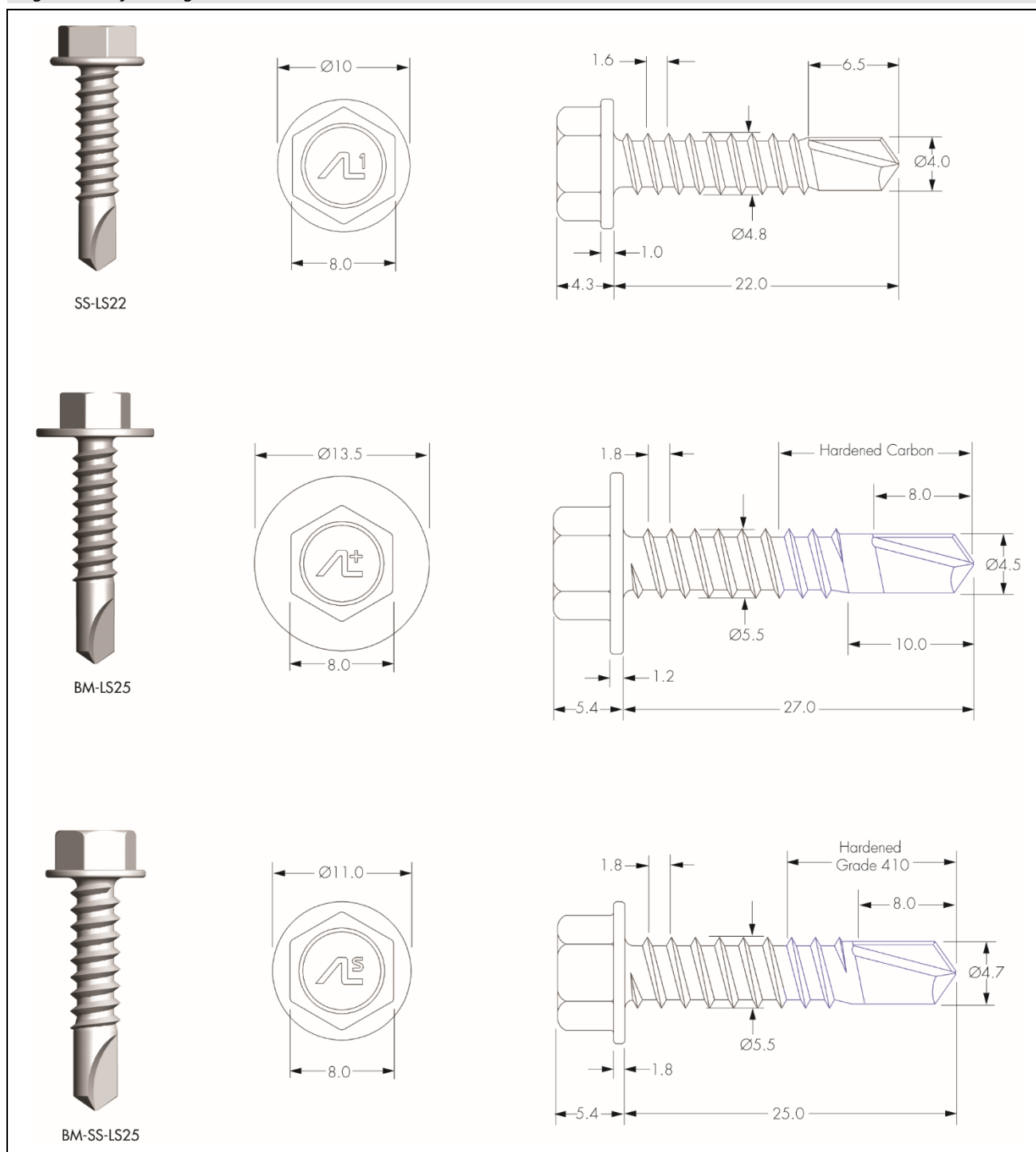
Figure 7 Self-drilling screws
