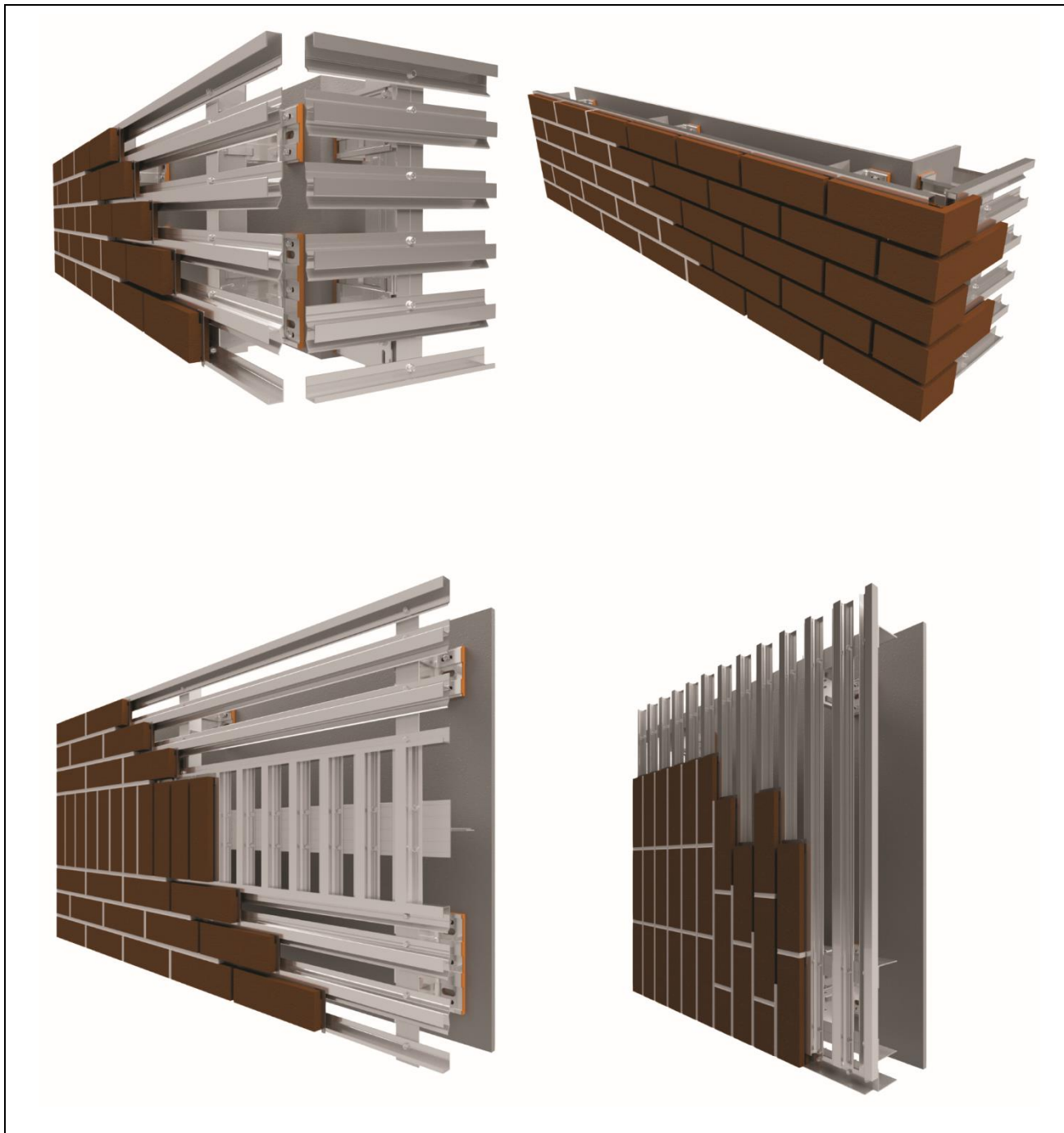
Figure 1 Mechslip System and AxiAL Supporting System
