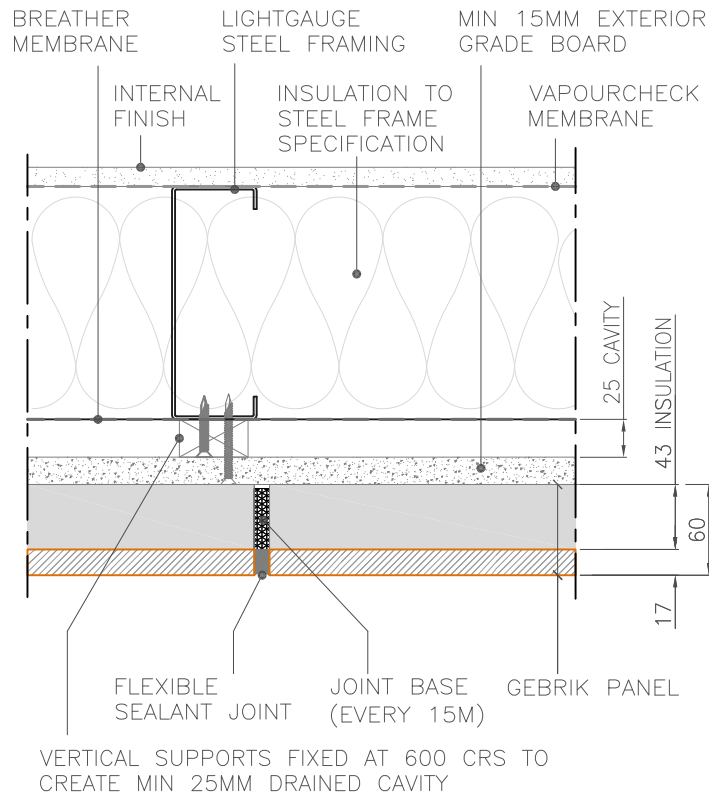
PLAN: VERTICAL JOINT
